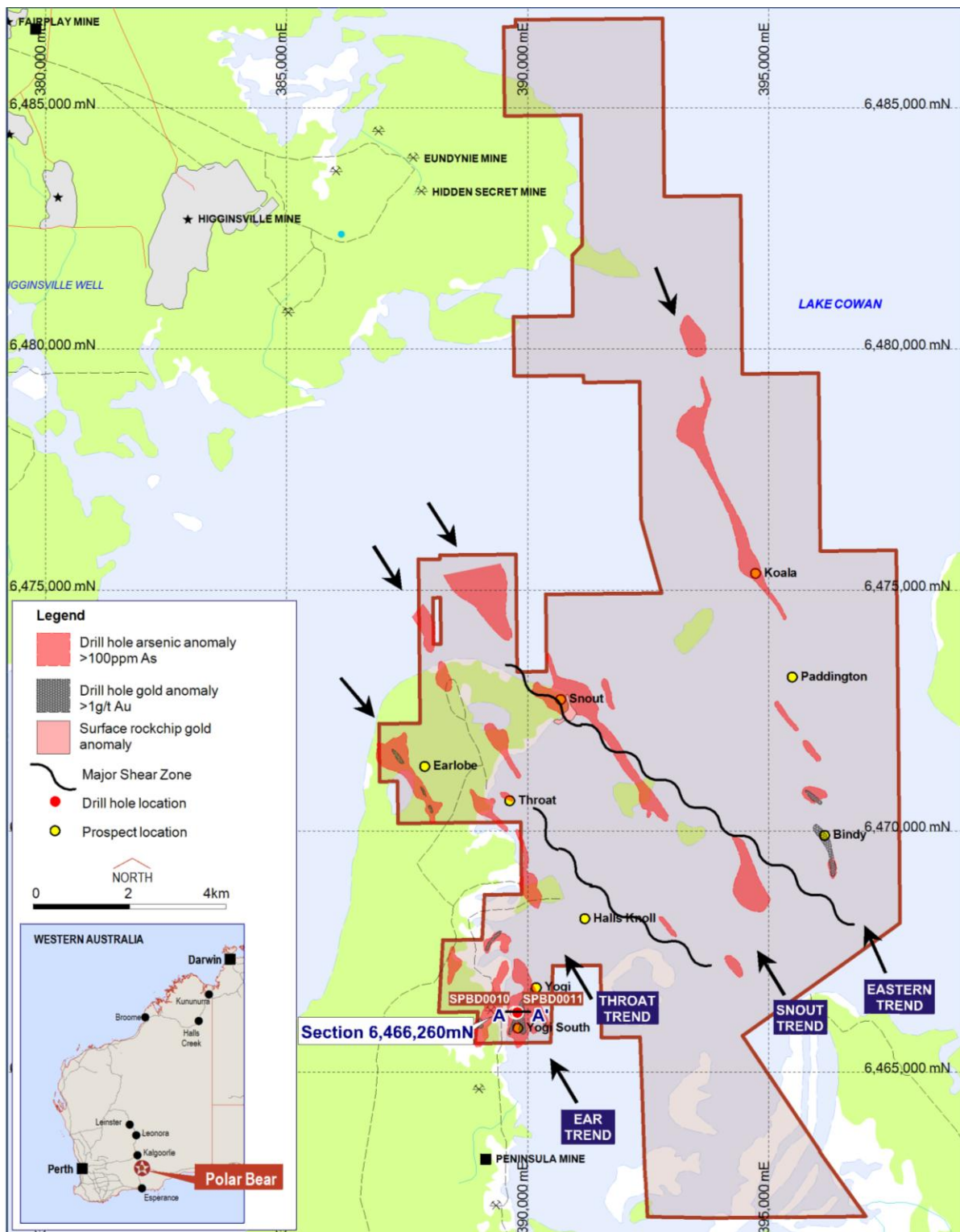
Figure 1. Location of Yogi prospect and associated gold anomalous trends along strike from Higgsville.
