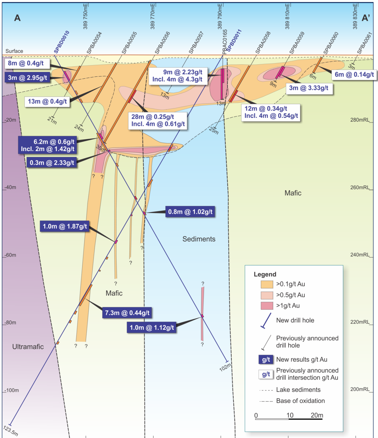
Figure 2. Cross section of Yogi prospect drilling, 6466260N.
